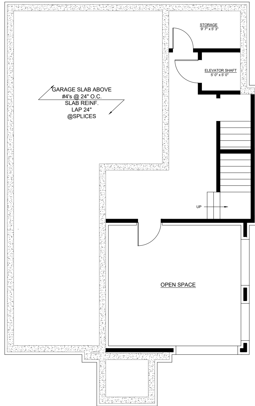
Basement Heated Area: 314 sqft Unheated Area: 306 sqft Total Heated Area: 3,326 sqft
