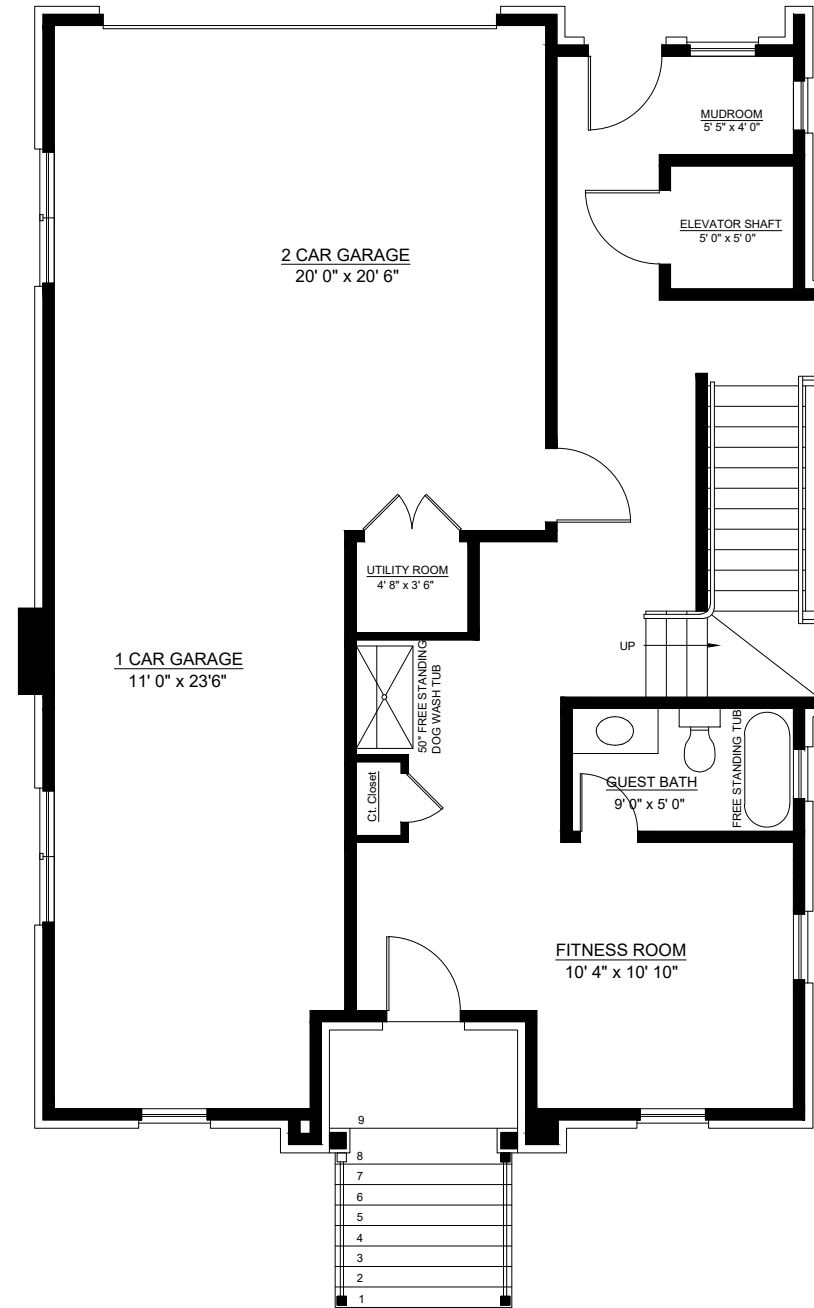
Lower Level Heated Area: 534 sqft Garage Area: 735 sqft Total Heated Area: 3,326 sqft
